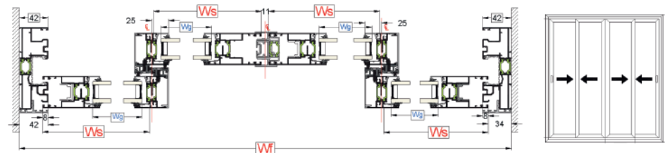
4 Pane Cross Section
